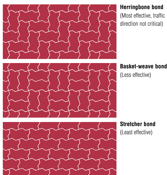
Figure 4 Laying patterns
