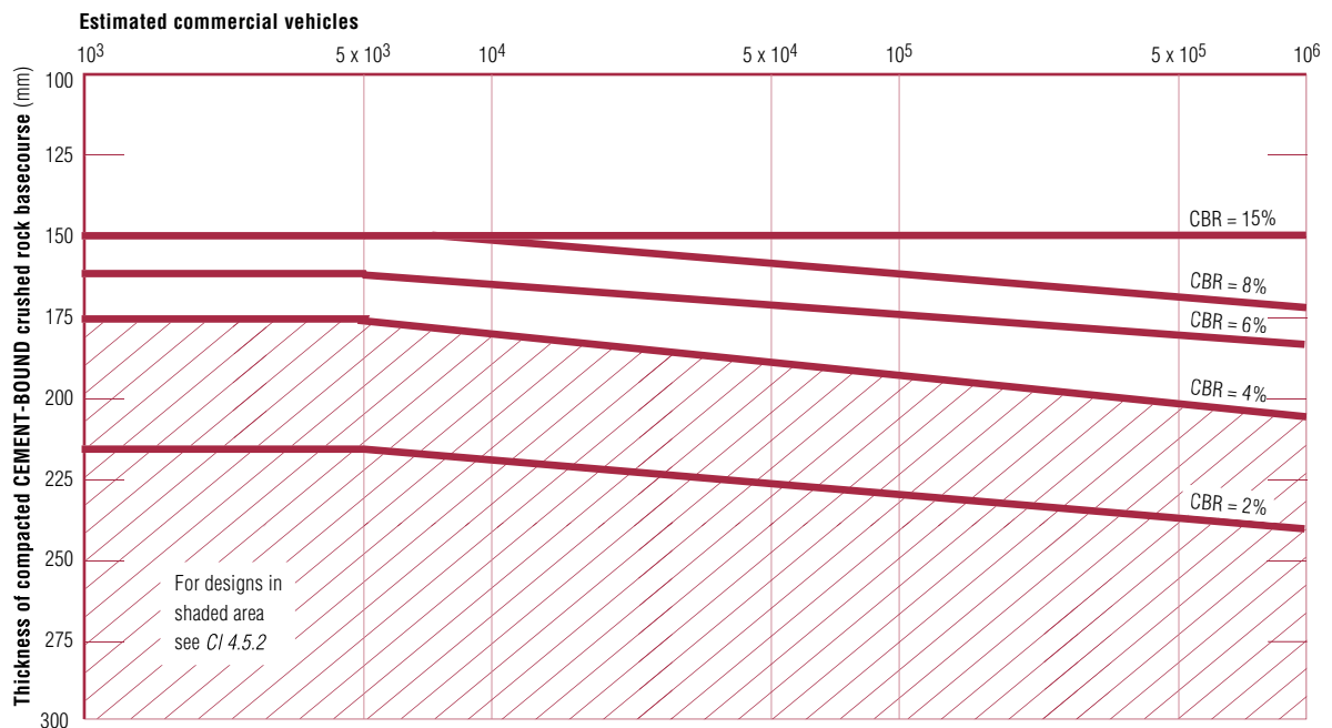
Figure 5 Example designs from LOCKPAVE
